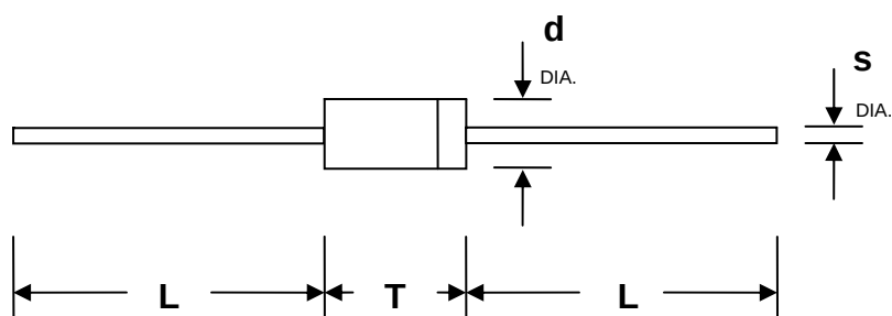
DO-201AL/DO-41
